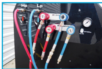
DOUBLE CONNECTOR SYSTEM R134a AND HFO1234yf
